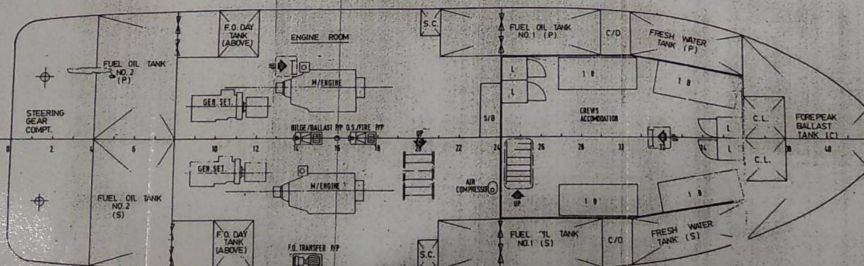
UNDER DECK PLAN
